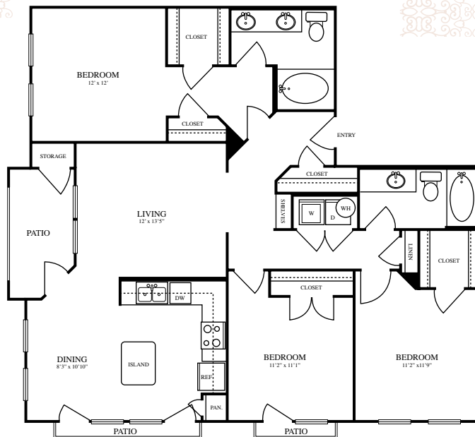
C1 1,326 SQFT THREE BEDROOM • TWO BATH
